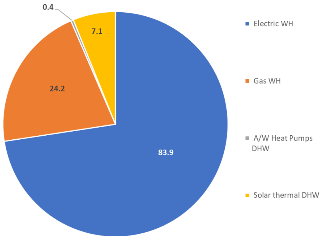
Figure 15 Water heating overall installed capacity in Germany in 2017 [GW]
