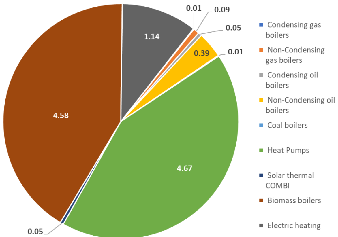
Figure 27 Space heating combi/space heating final energy consumption in Portugal in 2017 [TWh]
