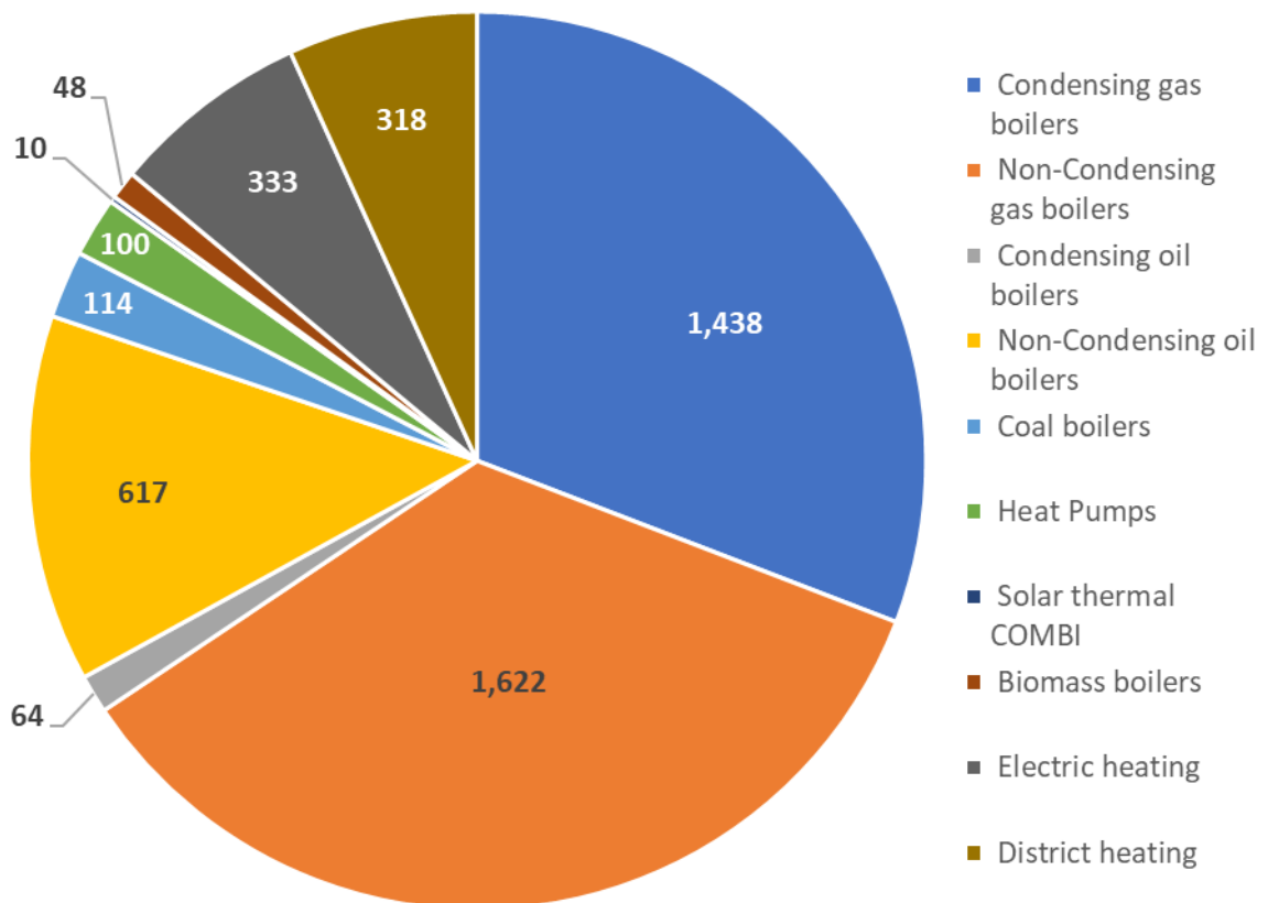
Figure 42 Space heating combi/space heating overall installed capacity in the EU in 2017 [GW]
