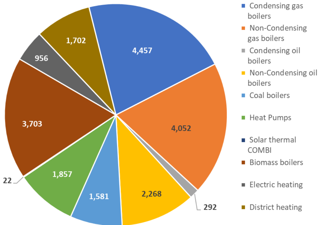
Figure 44 Space heating combi/space heating heated living area in the EU in 2017 [Mm 2 ]
