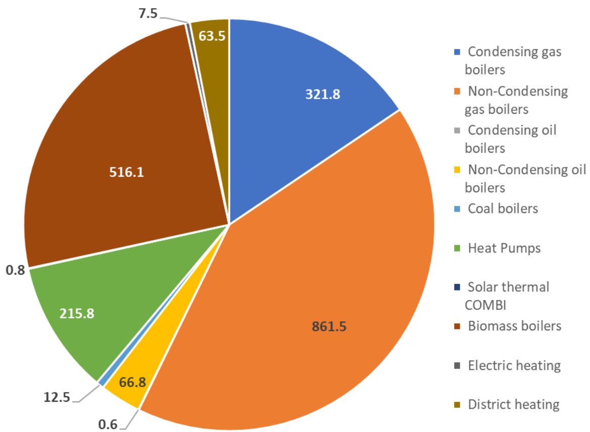
Figure 20 Space heating combi/space heating heated living area in Italy in 2017 [Mm 2 ]
