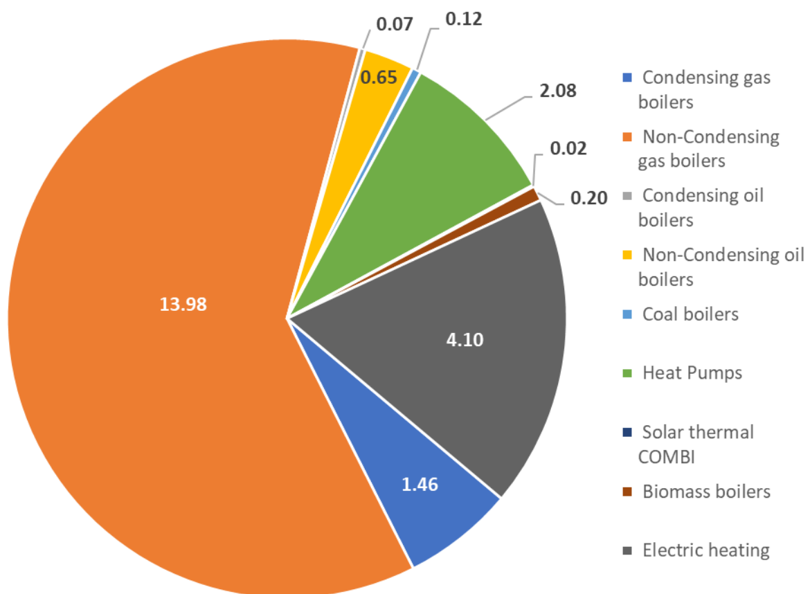
Figure 26 Space heating combi/space heating overall thermal capacity installed in Portugal in 2017 [GW]
