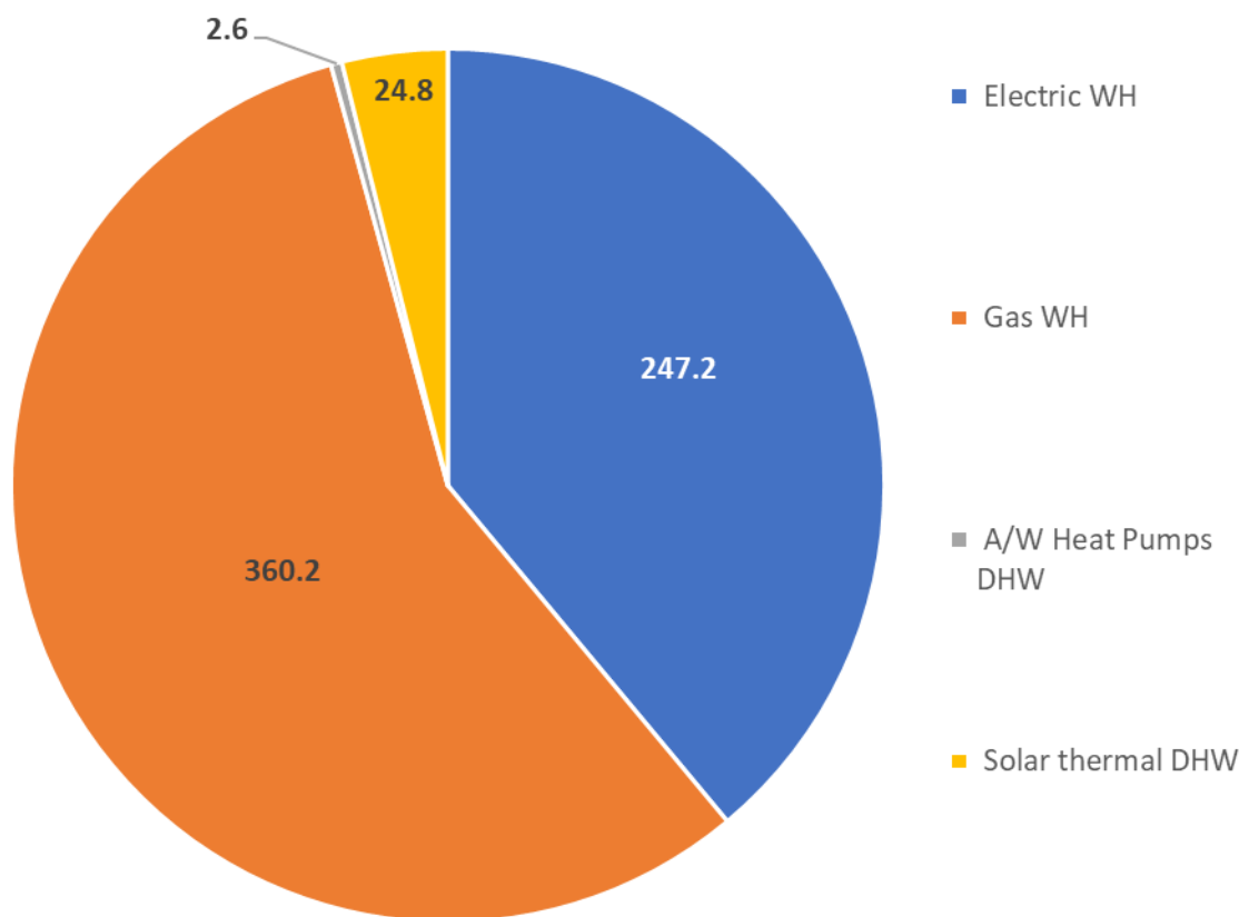
Figure 47 Water heating overall installed capacity in the EU in 2017 [GW]
