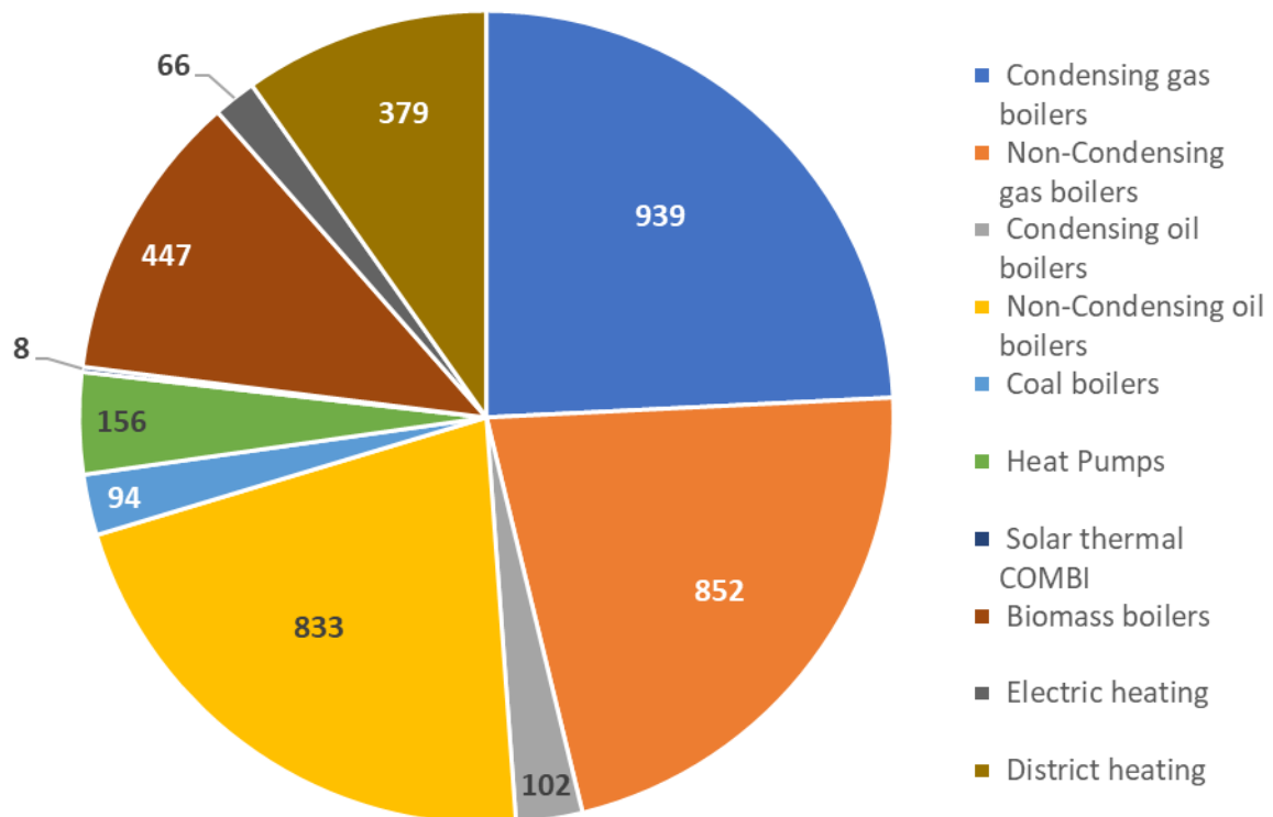
Figure 12 Space heating combi/space heating heated living area in Germany in 2017 [Mm 2 ]
