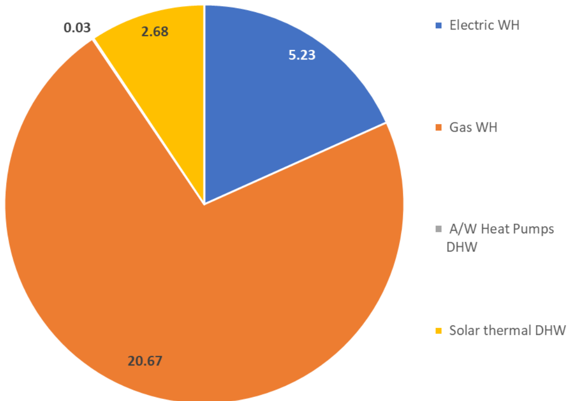
Figure 40 Water heating final energy consumption in Spain in 2017 [TWh]
