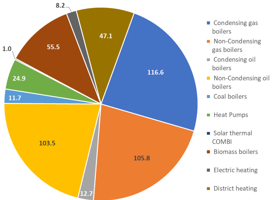
Figure 11 Space heating combi/space heating final energy consumption in Germany in 2017 [TWh]
