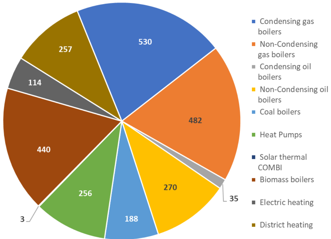
Figure 43 Space heating combi/space heating final energy consumption in the EU in 2017 [TWh]
